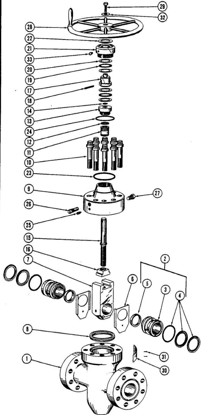
10,000 psi Type B Valve
